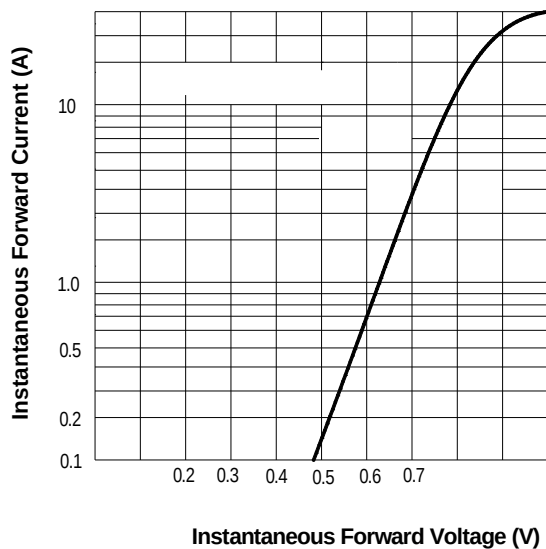
FIG3: Forward Voltage
