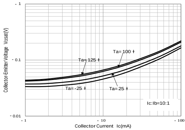
Collector-Emmitter Saturation Voltage
