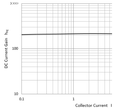
DC Current Gain h_{FE}
