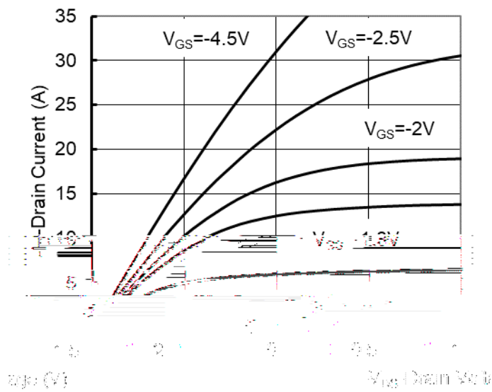
Figure1. Output Characteristics
