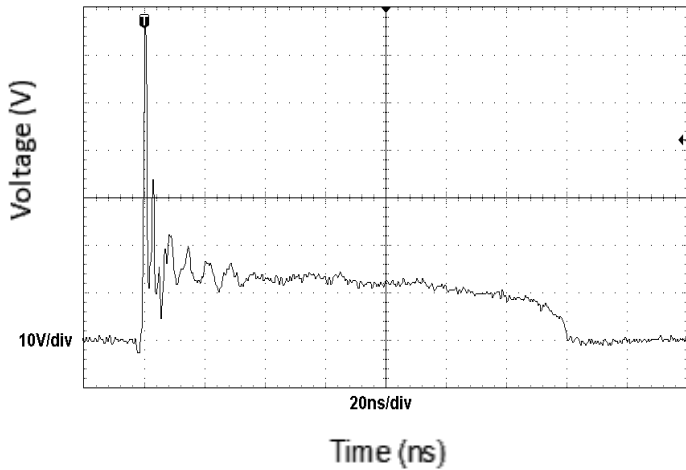
Fig.9 TLP Measurement
